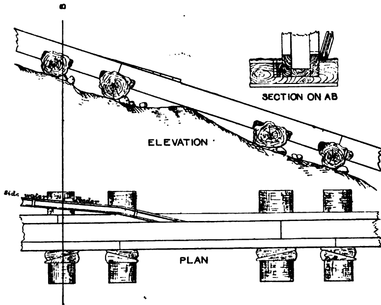
Fig. 202.—Deota sleeper slide.
